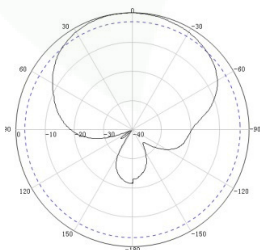
Horizontal Pattern
