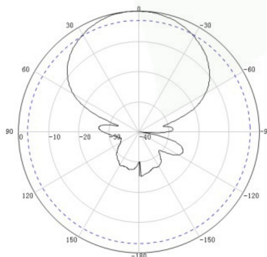
Vertical Pattern
